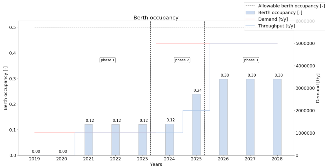
Figure E2.4: Berth occupancy
