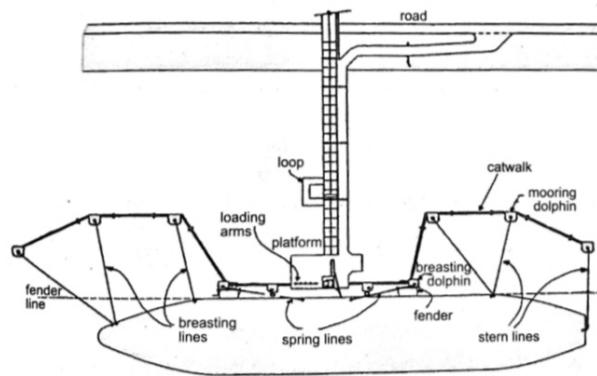
Figure 2.5: The design of a jetty from above (Ligteringen & Velsink, 2012)
