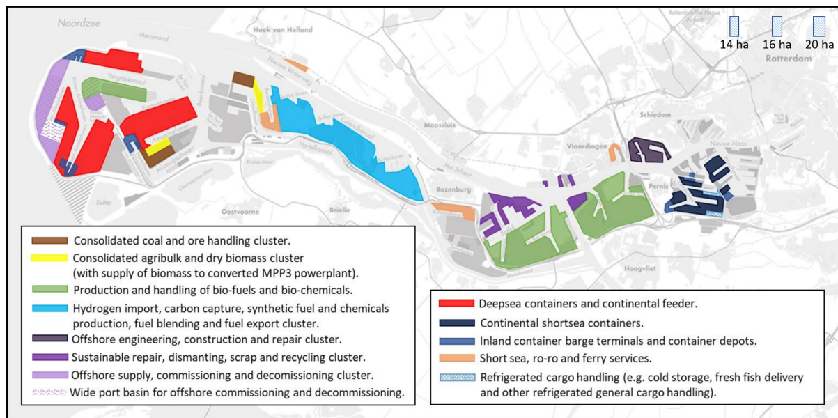
Figure 5.6: Outlined clustering of activities as suggested for the year 2040 with the indicated area for the import terminals (Van Dorsser, Taneja, & Vellinga, 2018)
