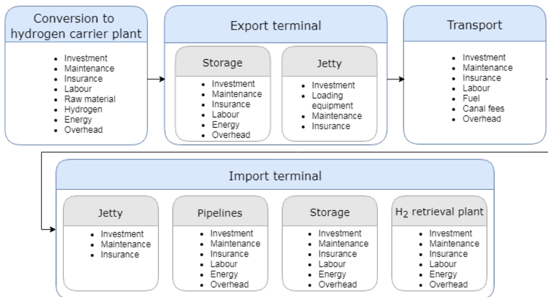
Figure 3.6: All possible supply chain elements from the model
