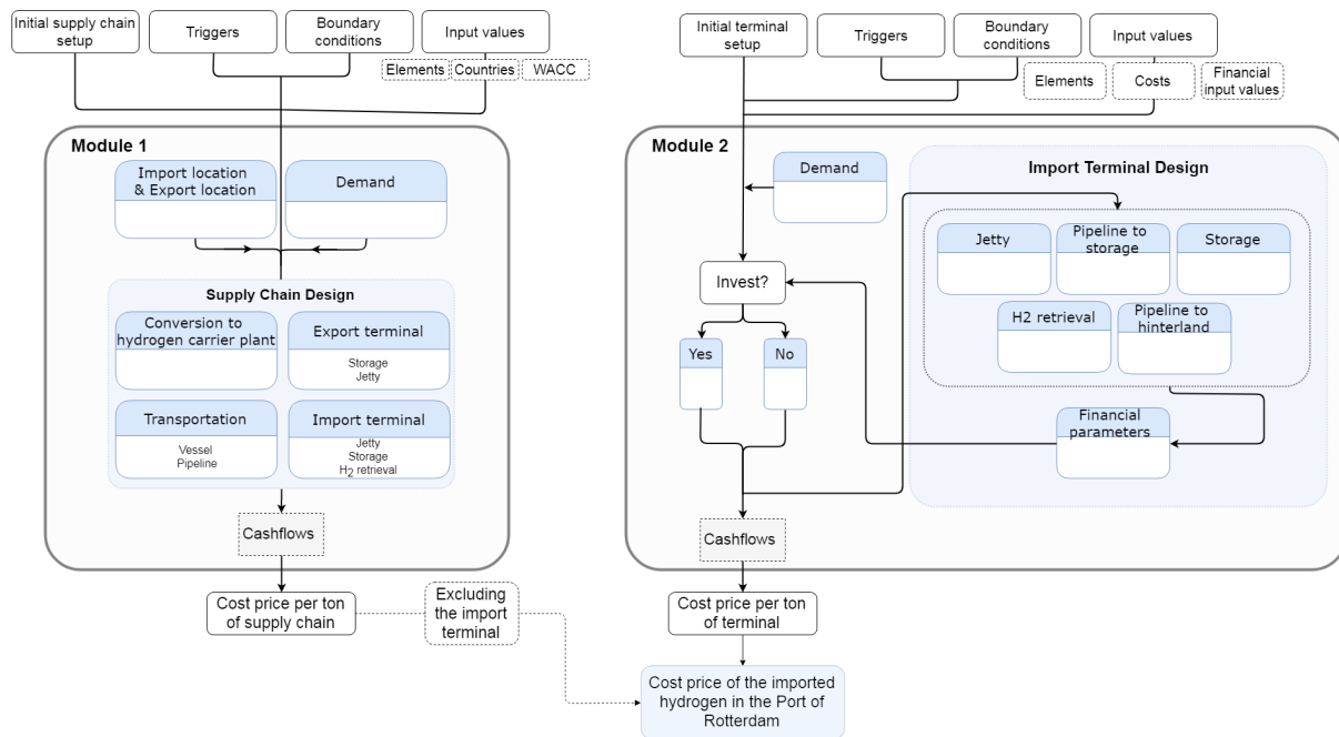
Figure 3.10: Model outline overview
