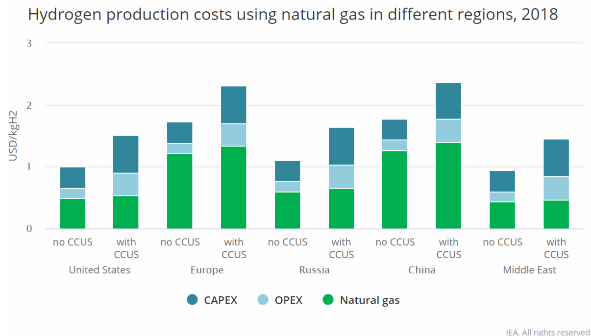
Figure B2.1: Hydrogen production costs using natural gas in different regions, 2018 (Birol, 2019)
