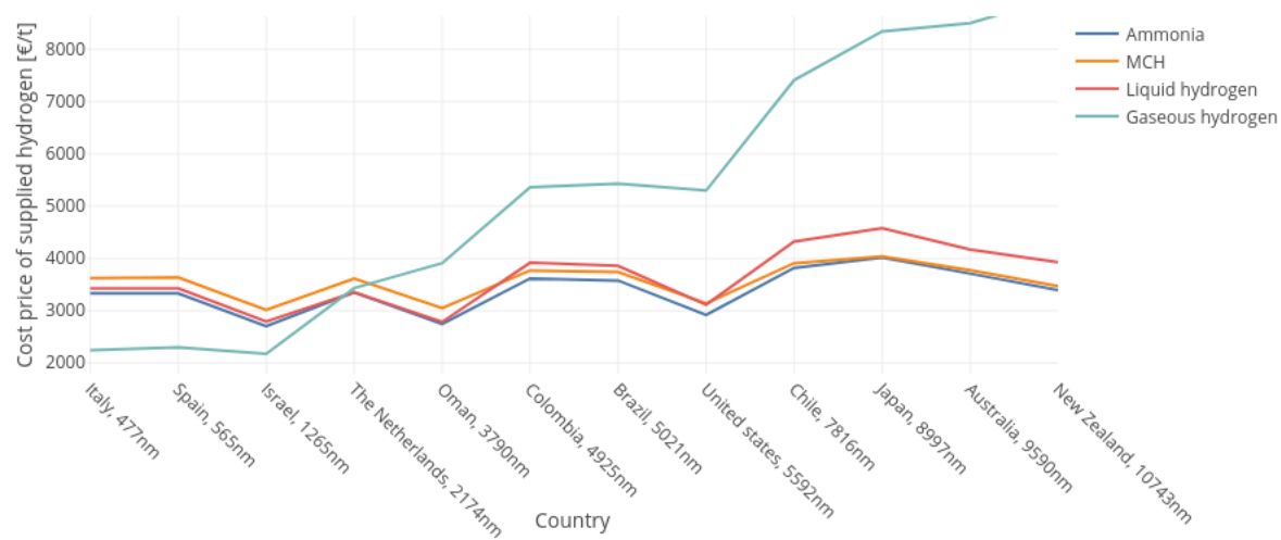
Figure F0.10: Cost price of the supplied hydrogen for the import in Tunisia varying with the countries, with a demand of 700,000 t/y
