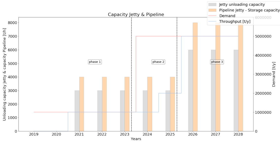
Figure E2.5: Capacity of the jetty to storage pipeline
