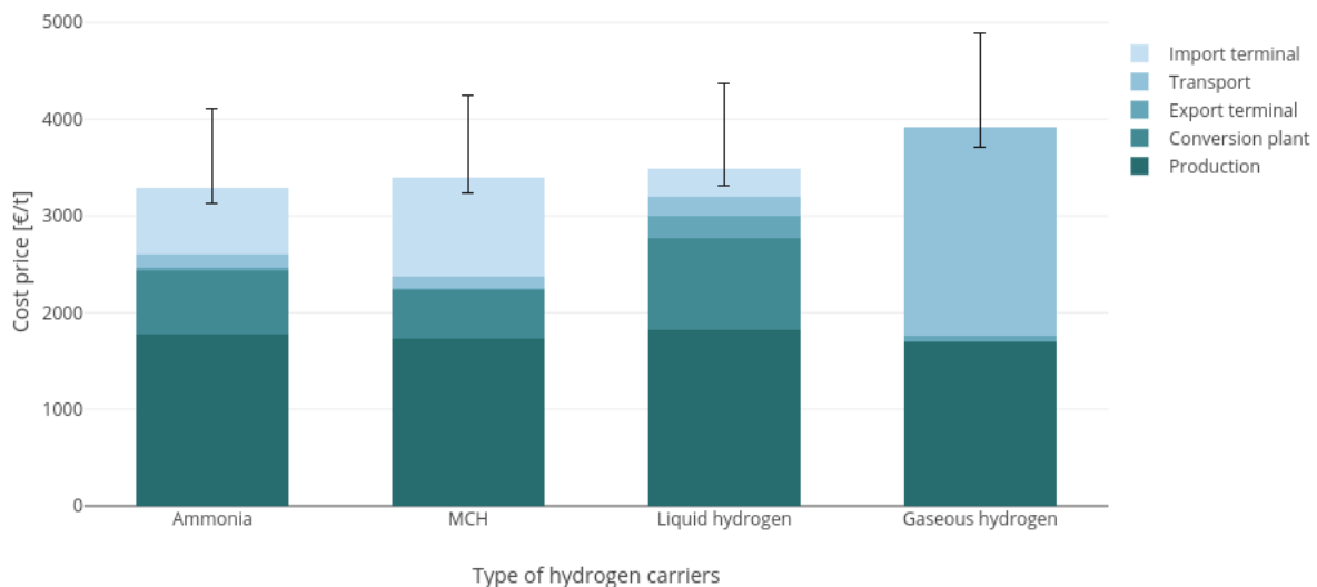
Figure 0.2: Cost price of the supplied hydrogen with a demand of 700,000 t/y, from Brazil to the Netherlands
