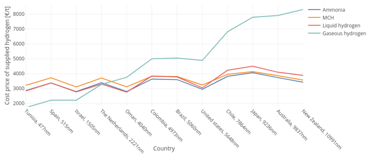
Figure F0.6: Cost price of the supplied hydrogen for the import in Italy varying with the countries, with a demand of 700,000 t/y
