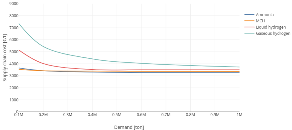
Figure 4.8: Cost price of the supplied hydrogen for the different hydrogen carriers
