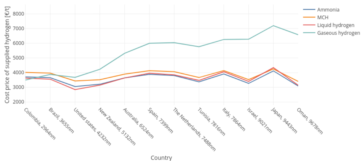
Figure F0.3: Cost price of the supplied hydrogen for the import in Chile varying with the countries, with a demand of 700,000 t/y
