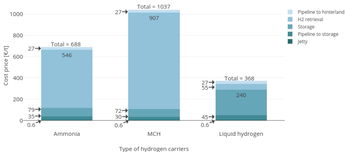
Figure 5.1: All the contributed costs (CAPEX and OPEX) of the elements of the import terminal, with a demand of 700,000 t/y
