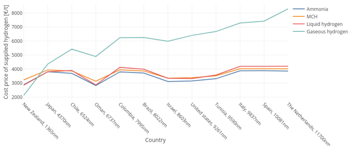
Figure F0.1: Cost price of the supplied hydrogen for the import in Australia varying with the countries, with a demand of 700,000 t/y
