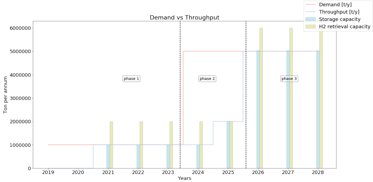
Figure E2.2: Throughput with bottleneck elements
