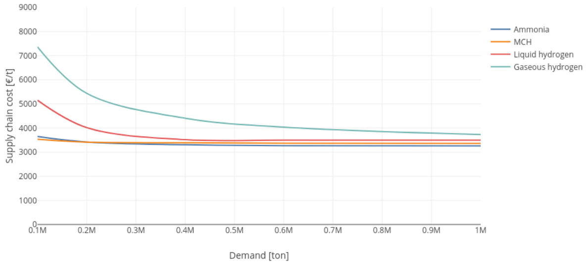
Figure 0.3: Cost price of the hydrogen supply chains varying with demand, from Brazil to the Netherlands
