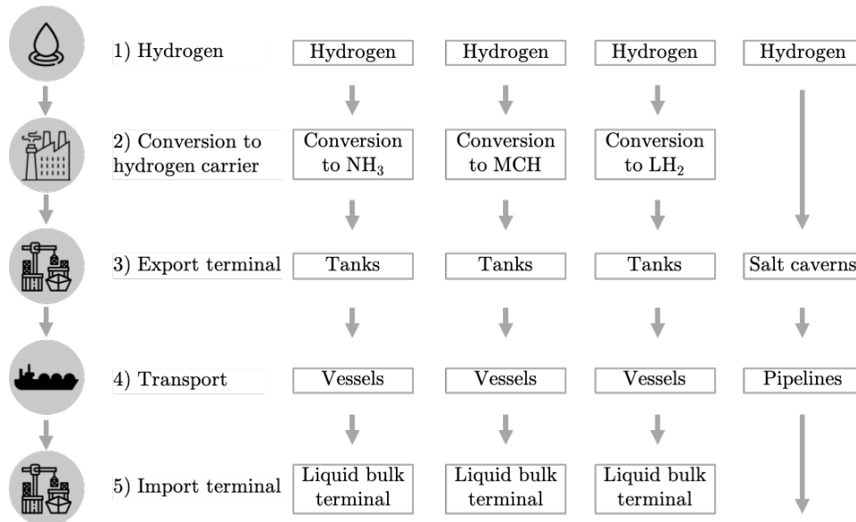
Figure 2.7: Supply chain of the different hydrogen carriers
