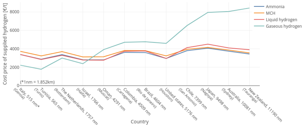
Figure 0.4: Cost price of the supplied hydrogen for the import in Spain varying with the countries, with a demand of 700,000 t/y
