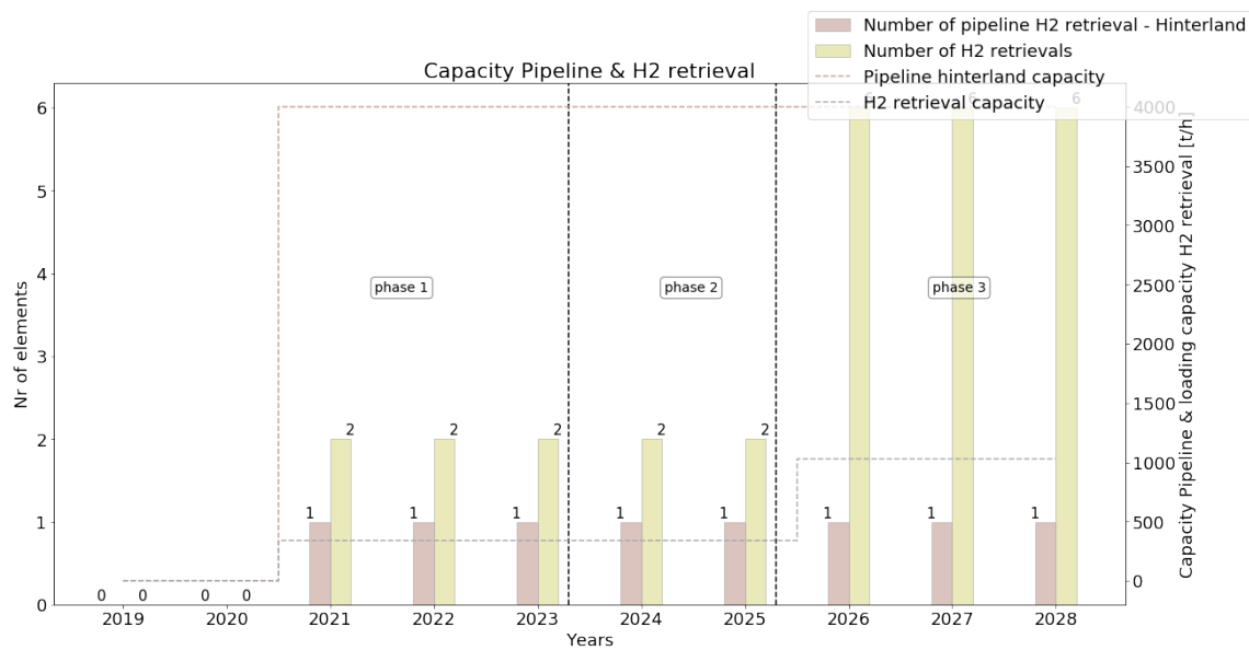
Figure E2.10: Number of pipelines [H 2 retrieval-Hinterland] with coherent capacity
