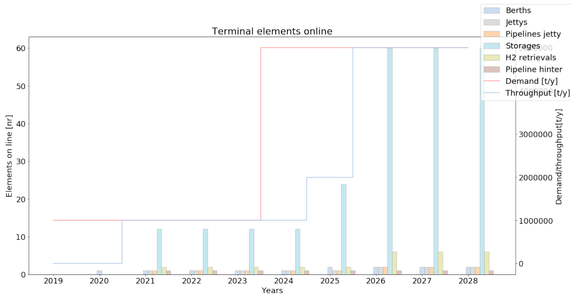
Figure E2.1: The elements of the terminal
