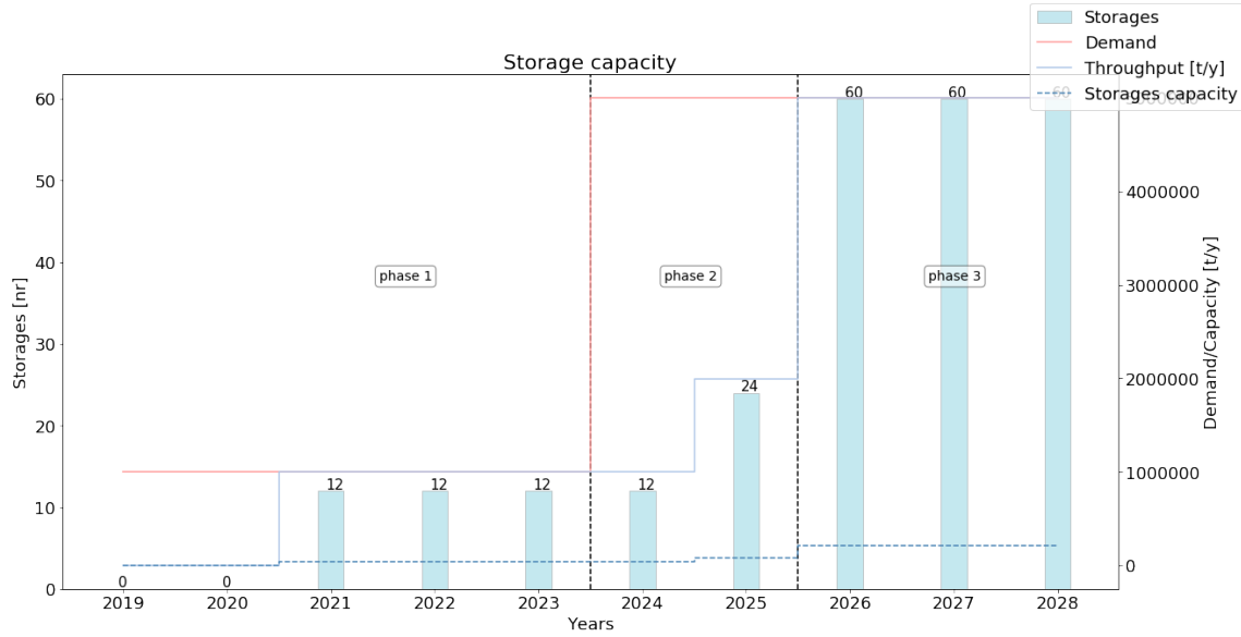
Figure E2.7: Number of storages with throughput
