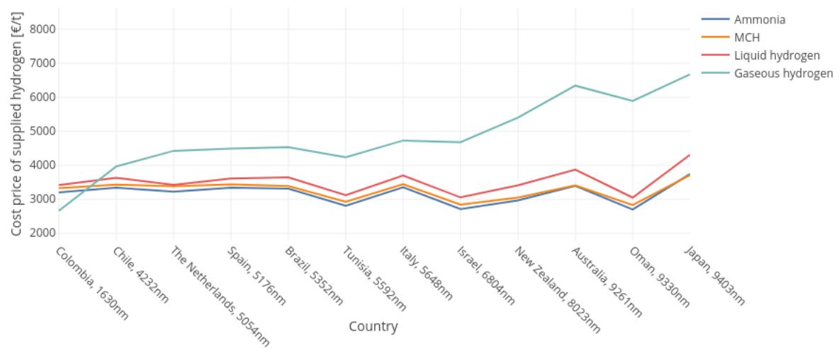
Figure F0.11: Cost price of the supplied hydrogen for the import in United States varying with the countries, with a demand of 700,000 t/y
