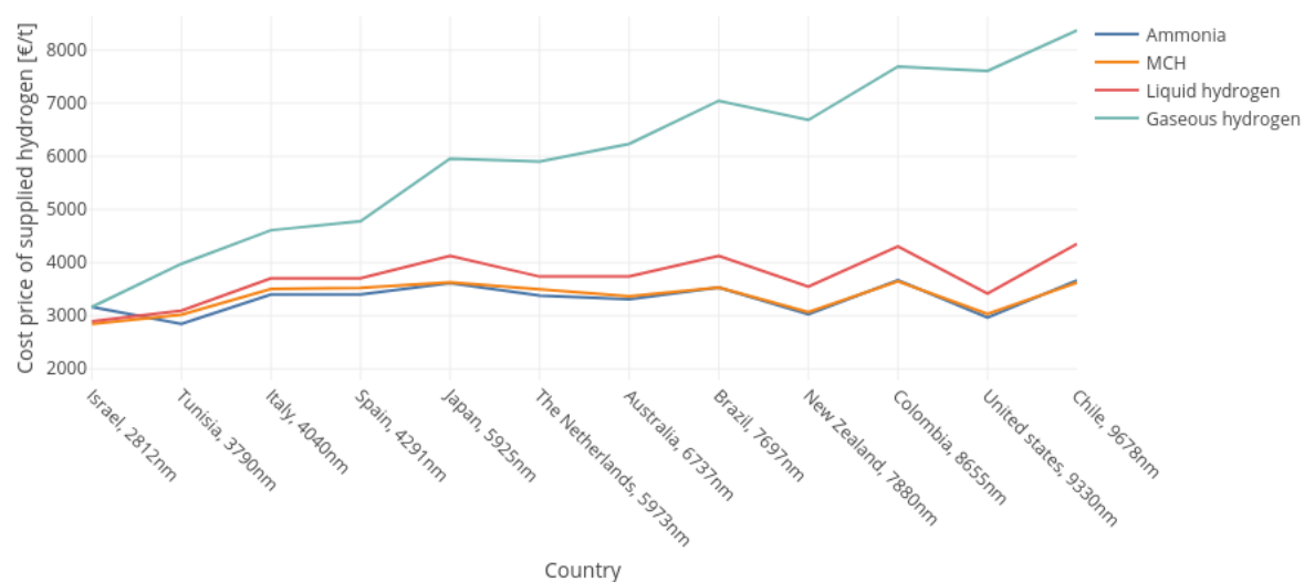
Figure F0.9: Cost price of the supplied hydrogen for the import in Oman varying with the countries, with a demand of 700,000 t/y
