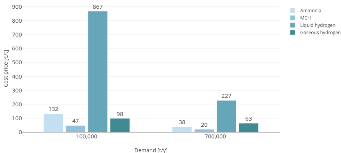
Figure 4.2: Cost price of the export terminal per hydrogen carrier
