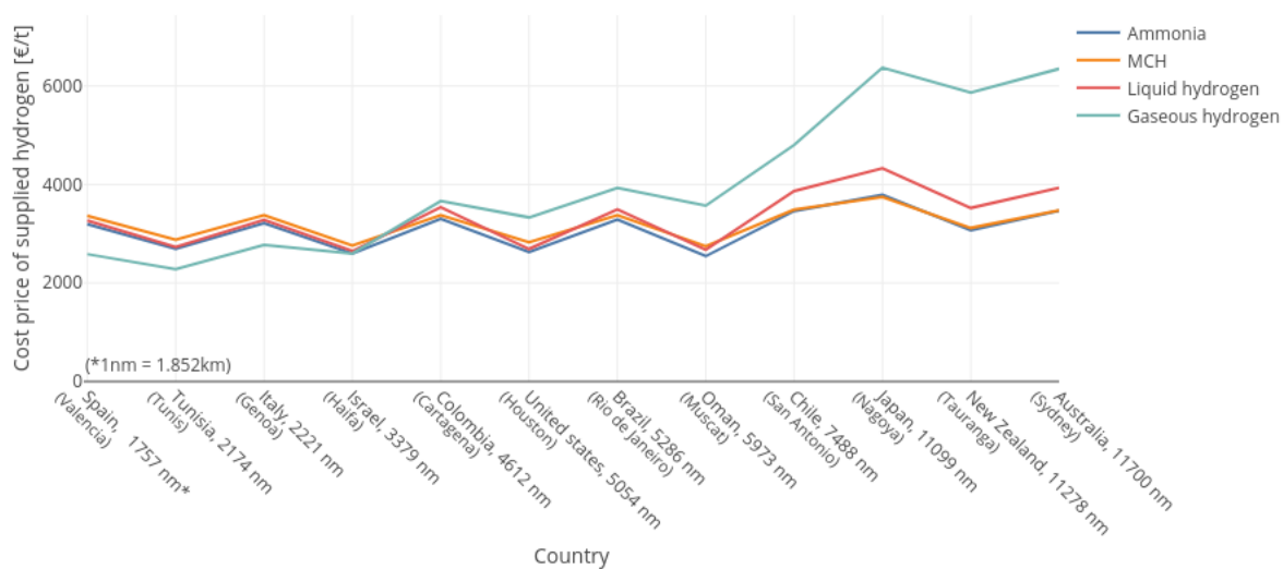
Figure 5.9: Cost price of the supplied hydrogen for importing in the Netherlands for the future hydrogen demand
