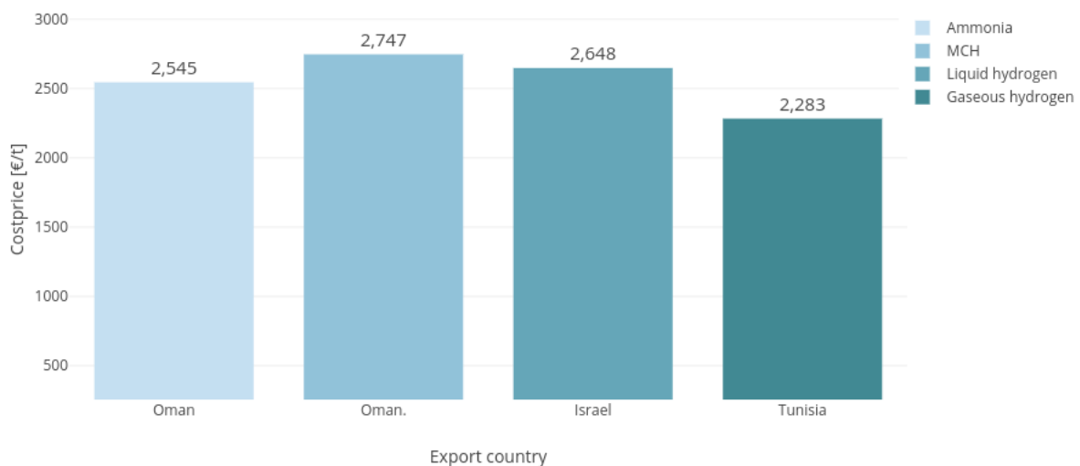
Figure 5.10: The optimal cost price of the hydrogen carriers combined with the export countries, for the import terminal in Rotterdam
