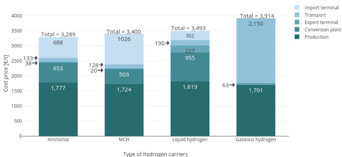
Figure 4.5: Cost price of the entire supply chain per hydrogen carrier with a demand of 700,000 ton, from Brazil to the Netherlands
