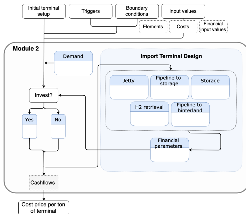
Figure 3.8: Overall outline of the import terminal investment model
