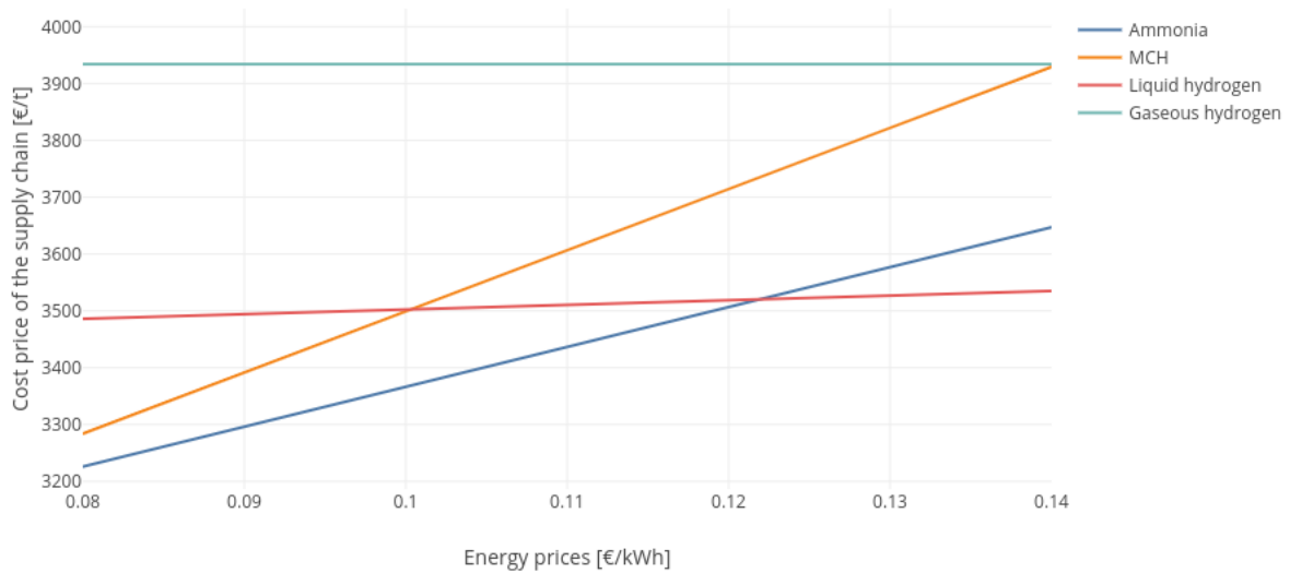
Figure 4.9: Cost price of the supplied hydrogen in combination with a varying energy price
