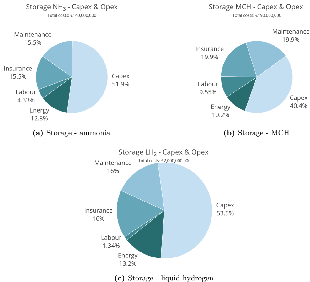
Figure 5.4: All the contributed costs of the storage for all carriers, based on the model output
