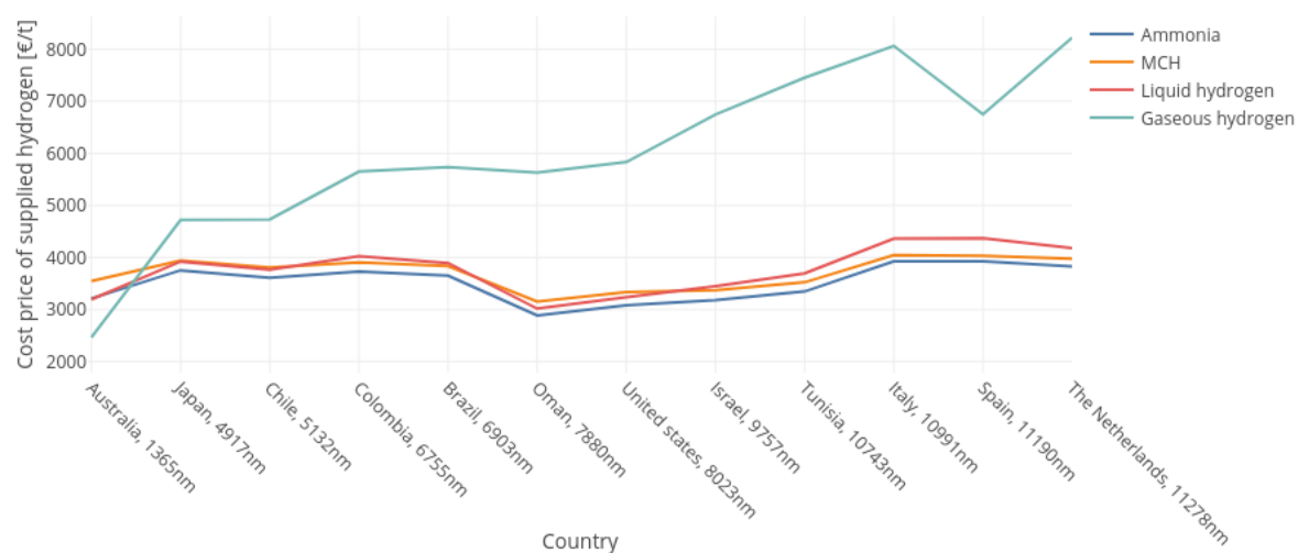
Figure F0.8: Cost price of the supplied hydrogen for the import in New Zealand varying with the countries, with a demand of 700,000 t/y
