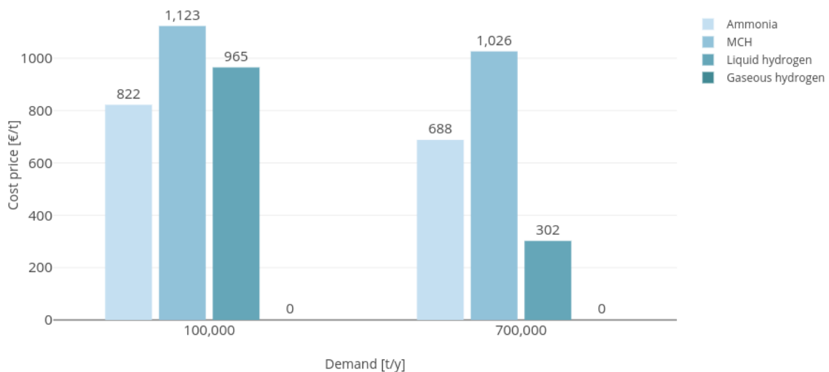
Figure 4.4: Cost price of the import terminal per hydrogen carrier
