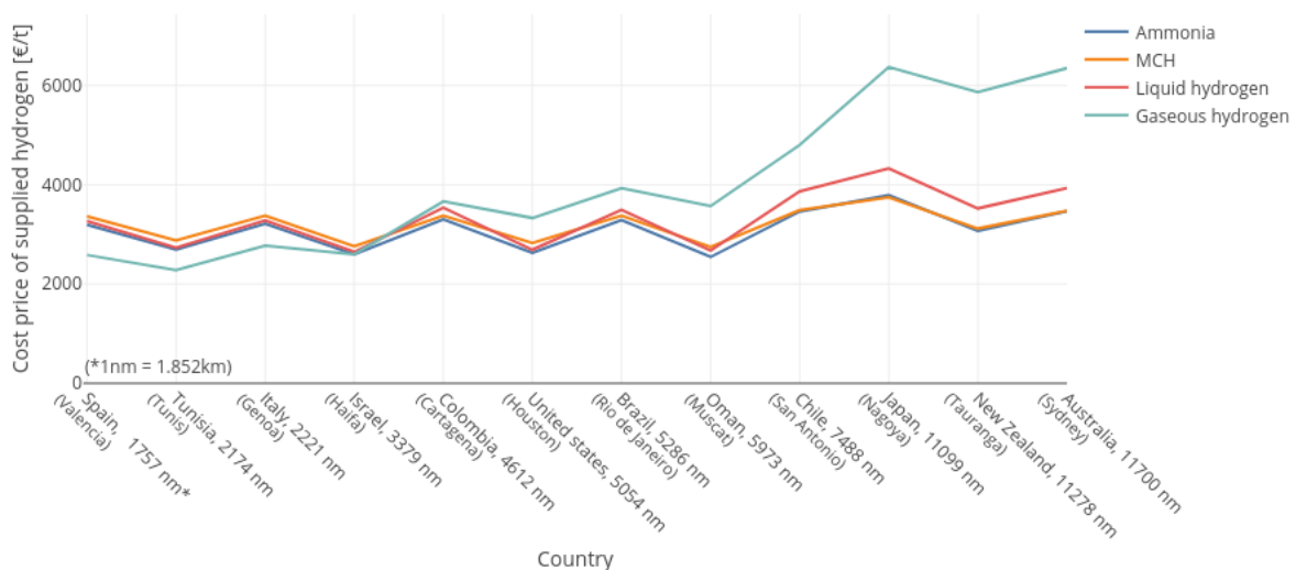
Figure 0.5: Cost prices of the supplied hydrogen for the import in the Netherlands
