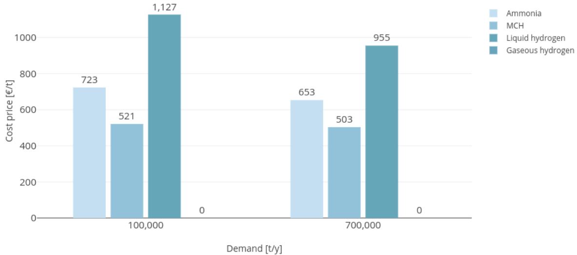
Figure 4.1: Cost price of the conversion plant per hydrogen carrier
