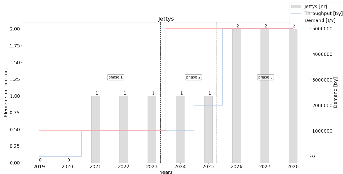
Figure E2.3: Number of jetties
