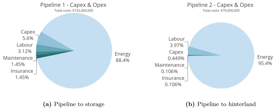
Figure 5.3: All the contributed costs of the pipelines for all carriers, based on the model output
