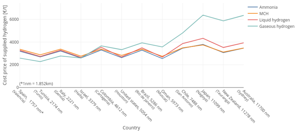
Figure 6.2: Cost prices of the supplied hydrogen for the import in the Netherlands
