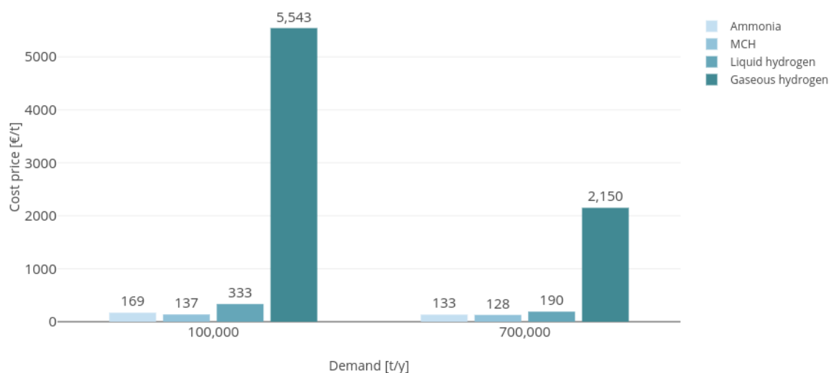
Figure 4.3: Cost price of the transportation per hydrogen carrier
