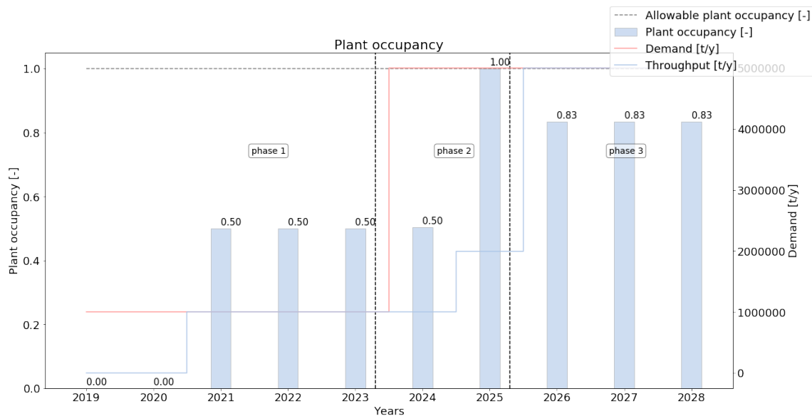
Figure E2.9: H 2 retrieval occupancy
