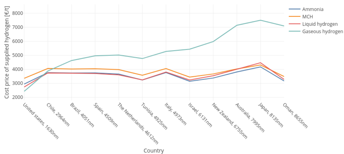
Figure F0.4: Cost price of the supplied hydrogen for the import in Colombia varying with the countries, with a demand of 700,000 t/y
