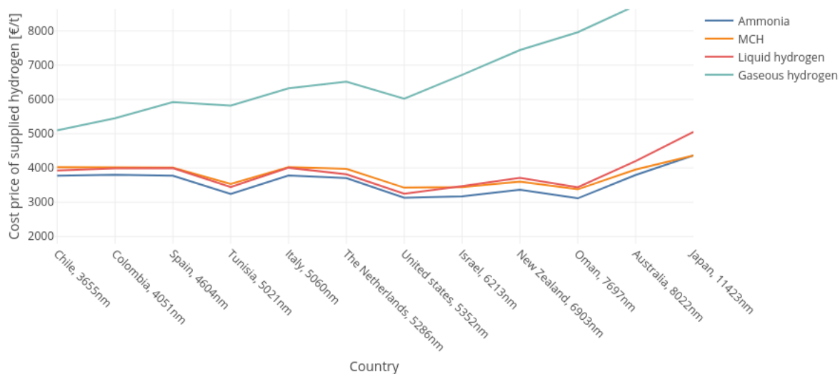
Figure F0.2: Cost price of the supplied hydrogen for the import in Brazil varying with the countries, with a demand of 700,000 t/y
