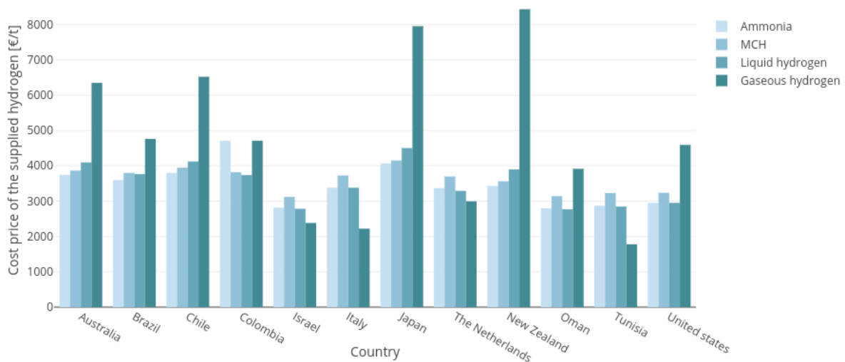
Figure 4.6: Cost price of hydrogen imported in Spain, with a demand of 700,000 t/y
