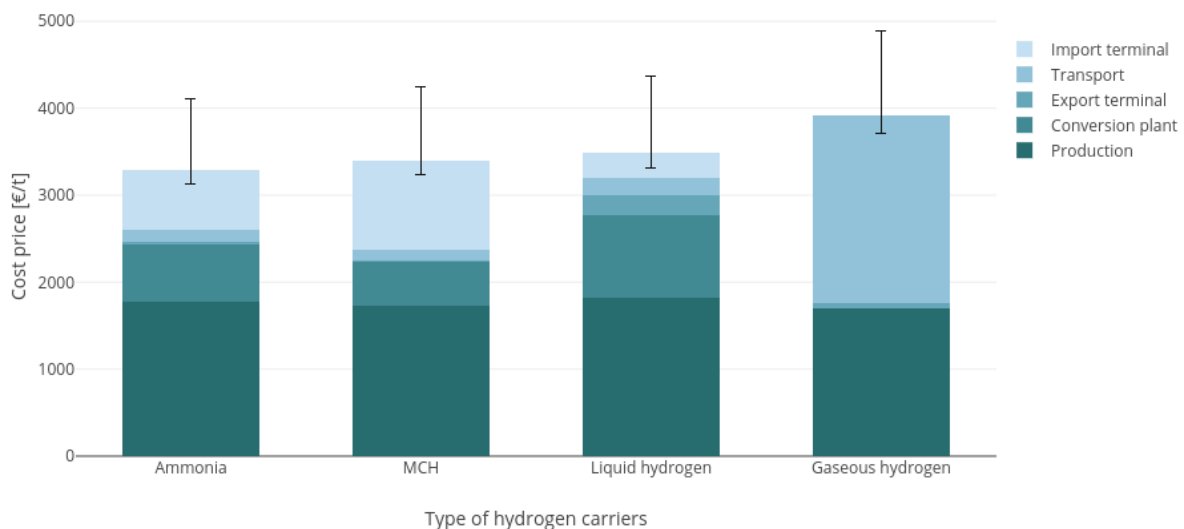
Figure 4.11: Cost price of the supplied hydrogen with a demand of 700,000 t/y, from Brazil to the Netherlands
