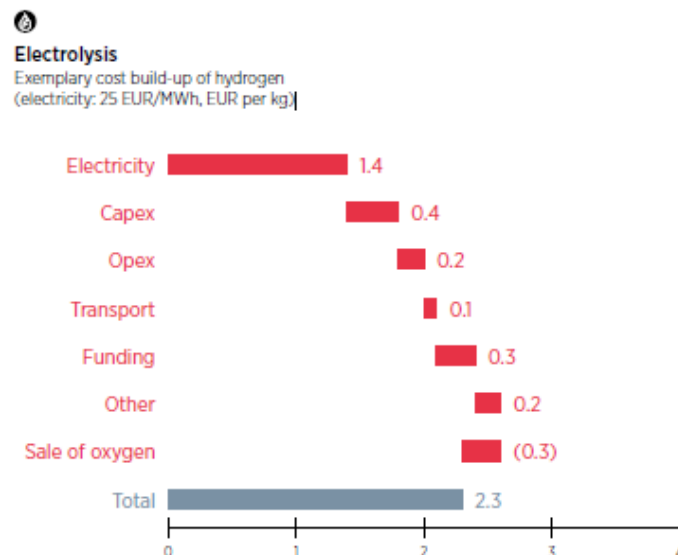
Figure A0.2: Exemplary cost build-up of hydrogen (Van Wijk, 2017)
