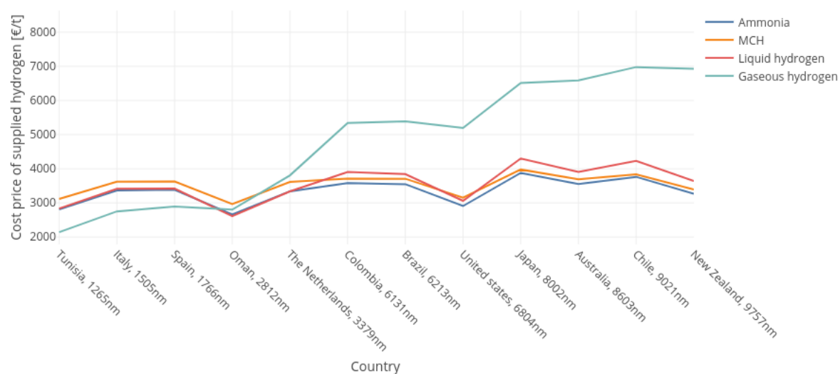
Figure F0.5: Cost price of the supplied hydrogen for the import in Israel varying with the countries, with a demand of 700,000 t/y
