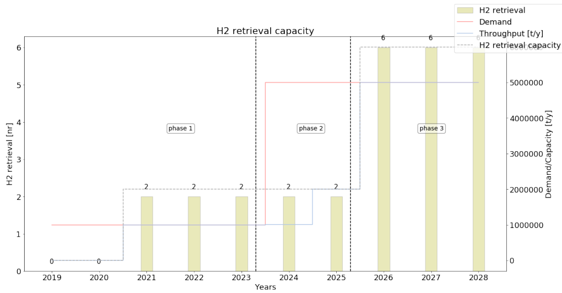
Figure E2.8: Number of H 2 retrieval's with coherent capacity
