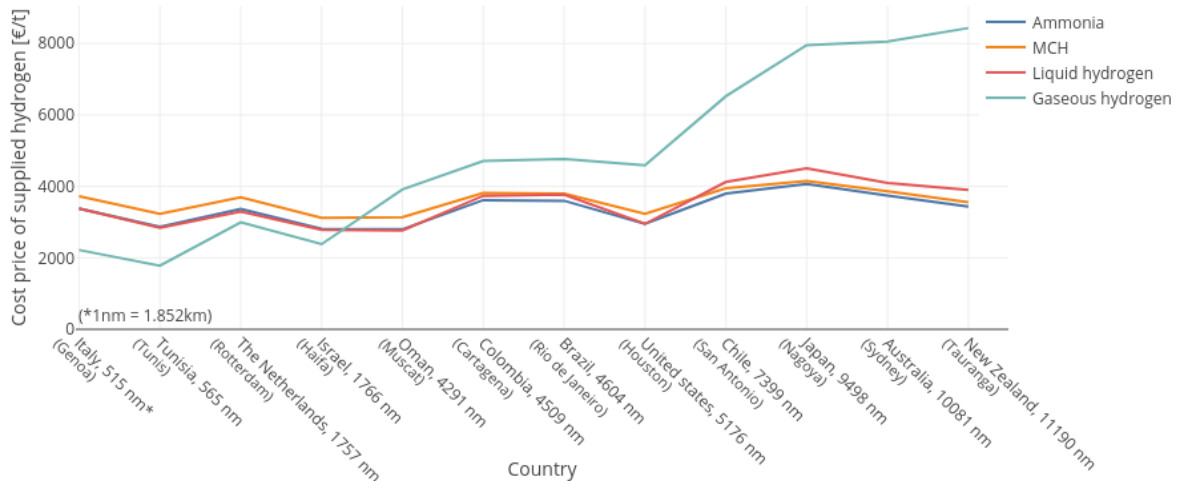
Figure 6.1: Cost price of the supplied hydrogen for the import in Spain with a demand of 700,000 t/y
