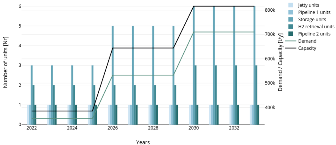
Figure E1.4: The development of the capacity of the import terminal
