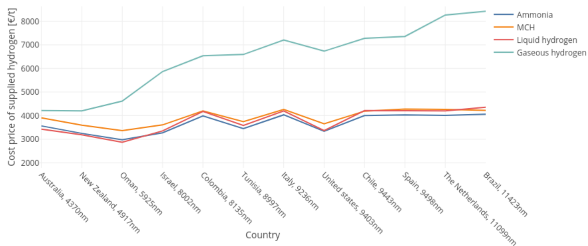
Figure F0.7: Cost price of the supplied hydrogen for the import in Japan varying with the countries, with a demand of 700,000 t/y
