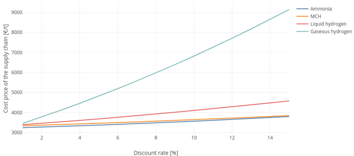
Figure 4.10: Cost price of the supplied hydrogen in combination with a varying discount rate
