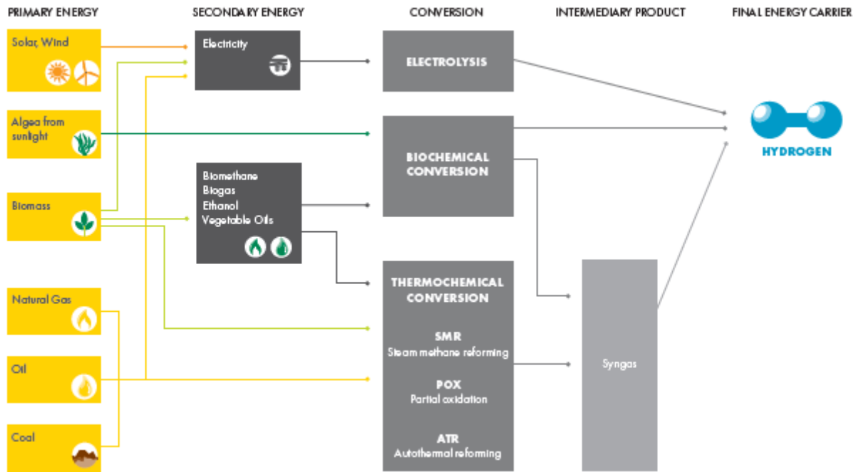
Figure A2.1: Processes for producing hydrogen (Shell Deutschland Oil GmbH, 2017)
