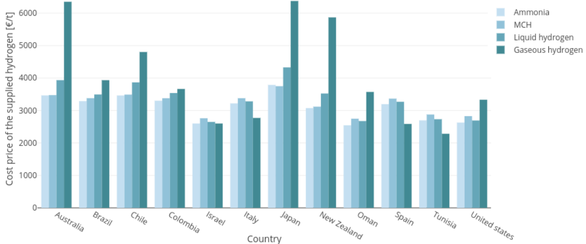
Figure 5.8: Cost price of the supplied hydrogen for the import in the Netherlands
