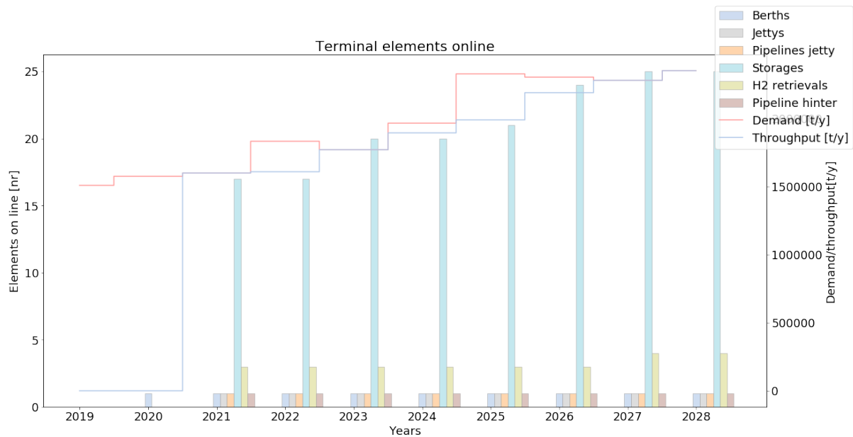
Figure 3.7: Terminal design
